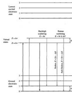
Figure 18-2 Origin of Rayleigh and Raman scattering
